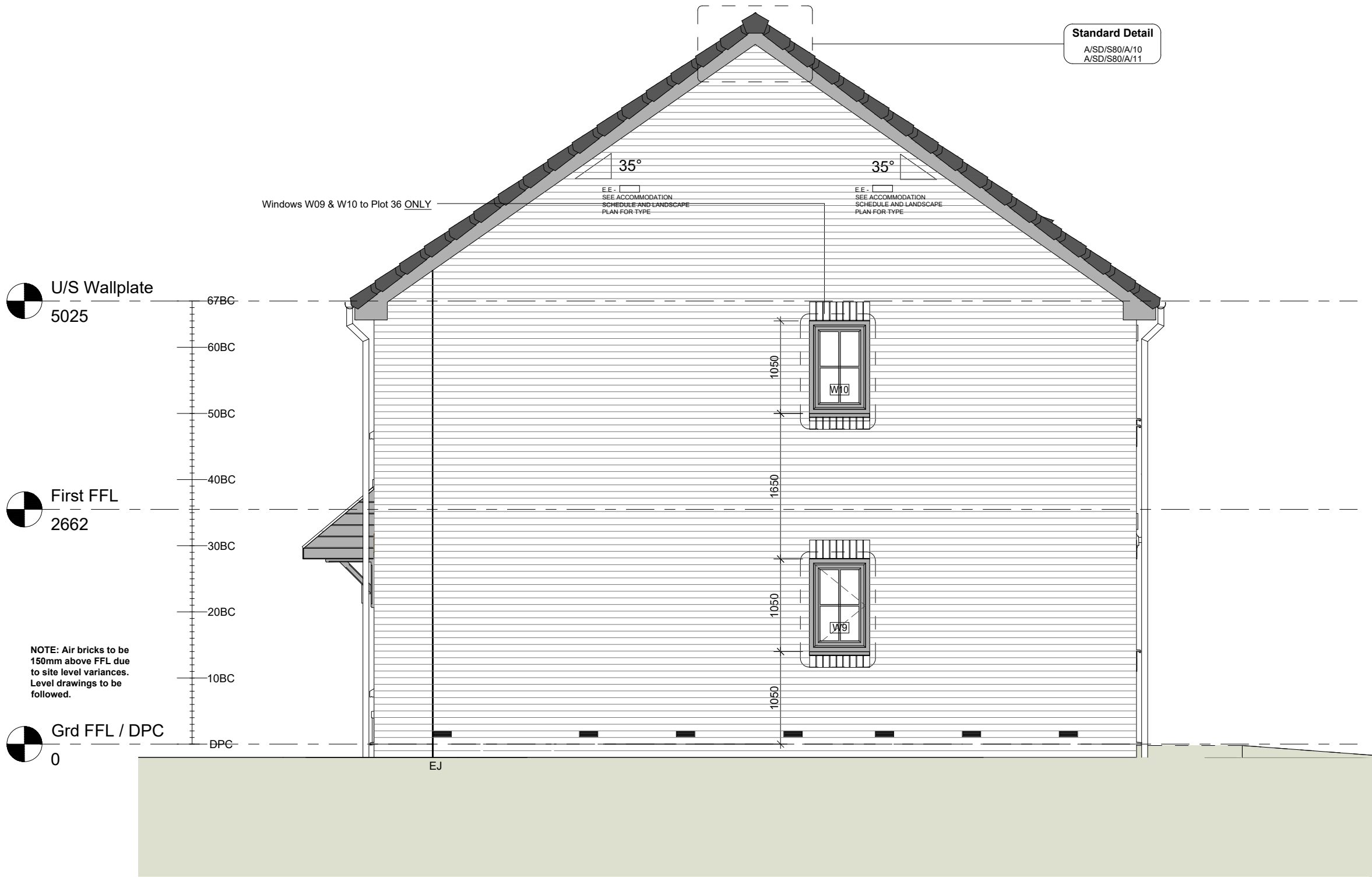
1 Gable Elevation 1 : 50
